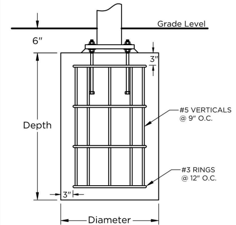
Auger Footing
