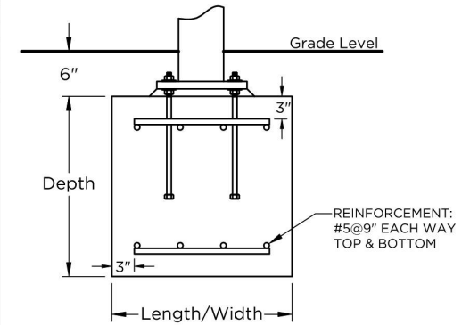
Square Footing
