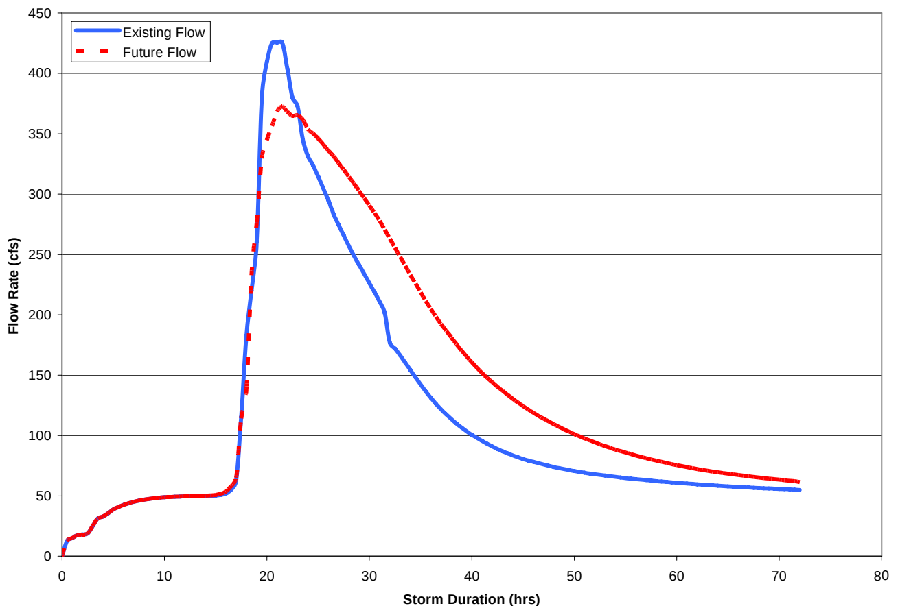
Figure 6-6 Example Hydrograph
