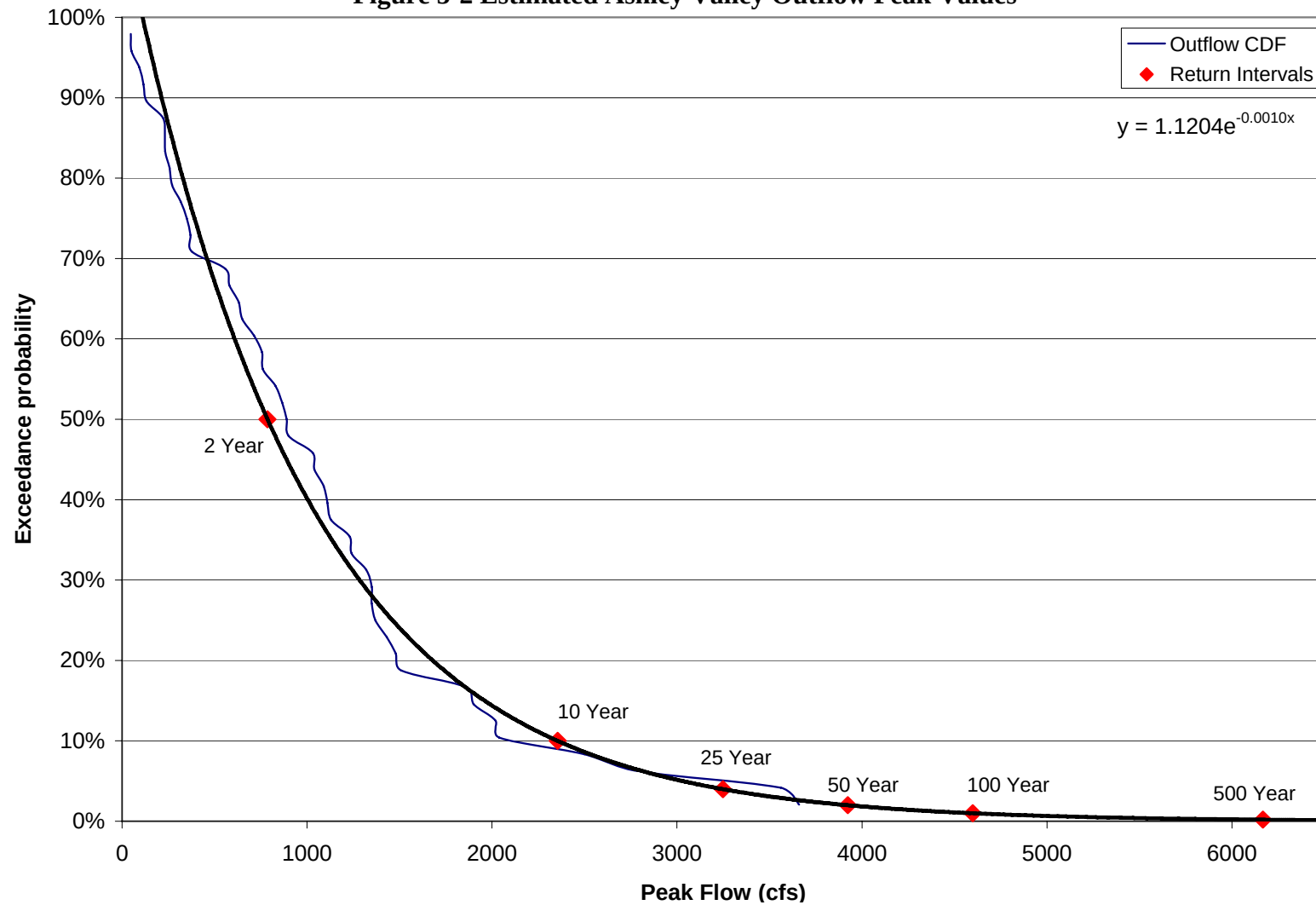
Figure 5-2 Estimated Ashley Valley Outflow Peak Values
