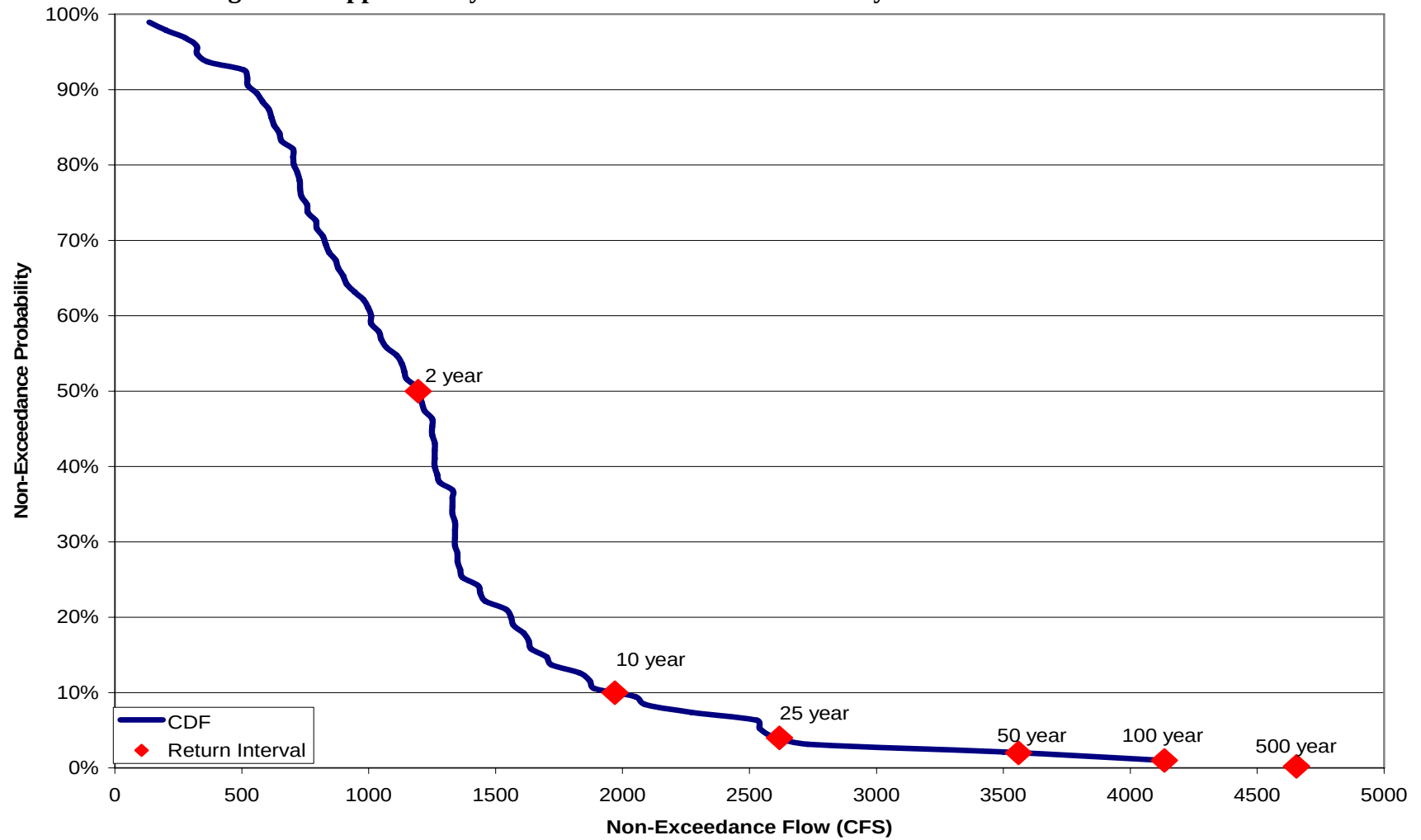
Figure 2-7 Upper Ashley Creek Non-Exceedance Probability Distribution Function
